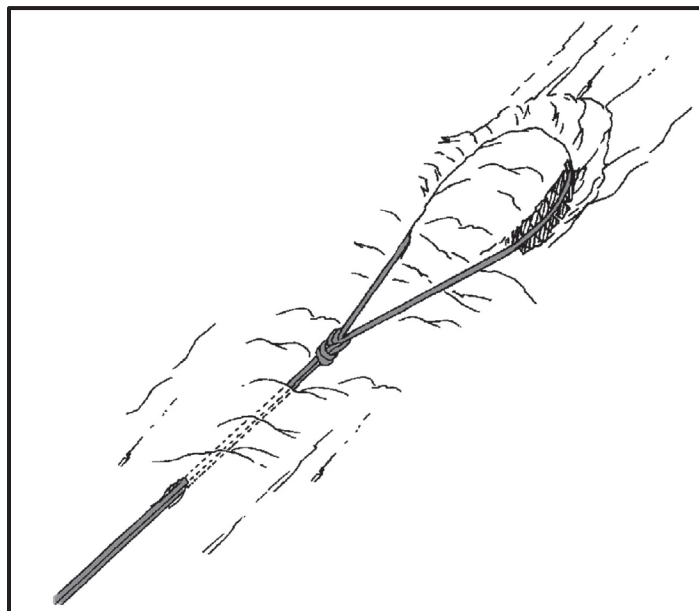
Figure 10-18. Horseshoe or bollard anchor.
