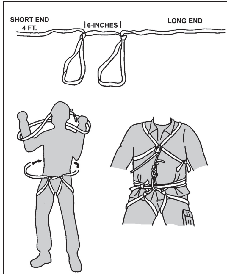
Figure 6-20. Improved seat and chest harness.
