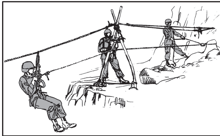
Figure 7-19. Suspension traverse.
