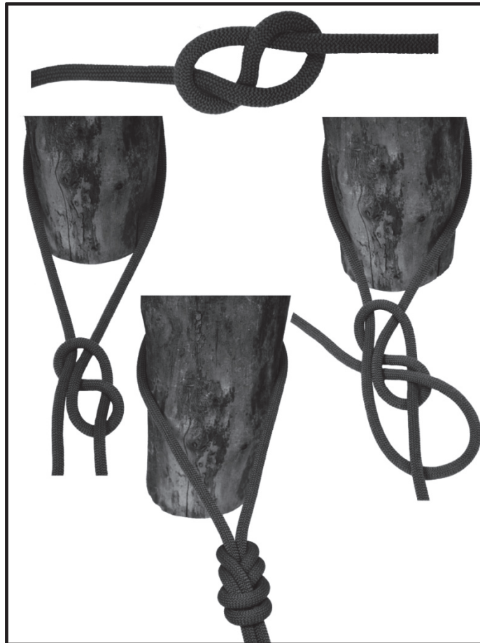
Figure 4-13. Figure-eight retrace.
