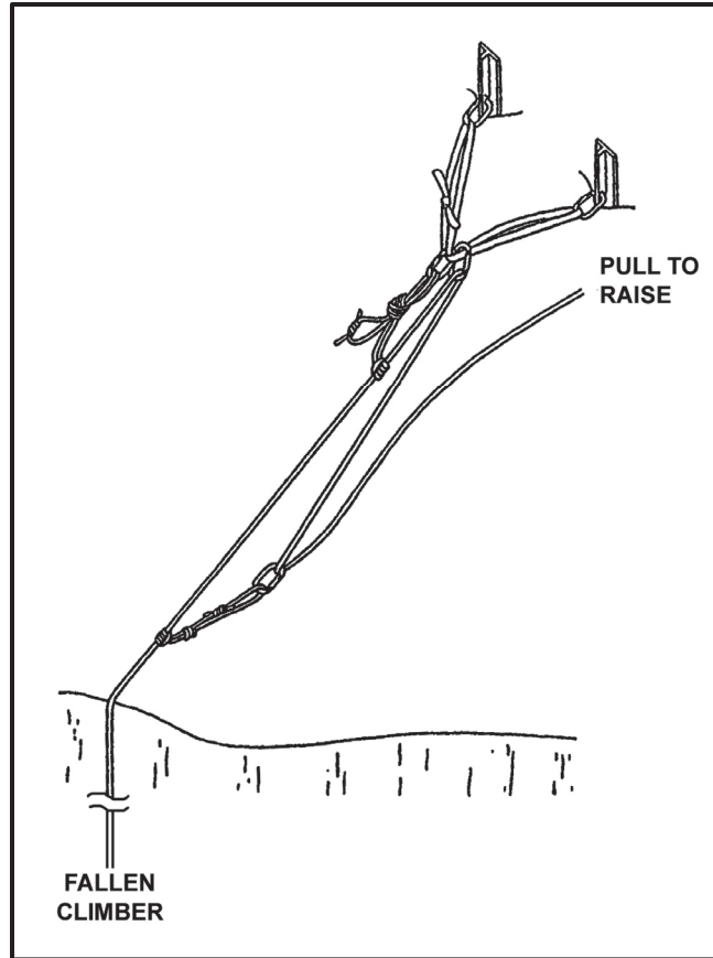
Figure 7-26. Z-pulley system.
