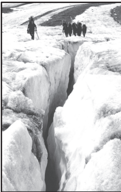
Figure 10-23. Ablation zone of glacier in summer.
