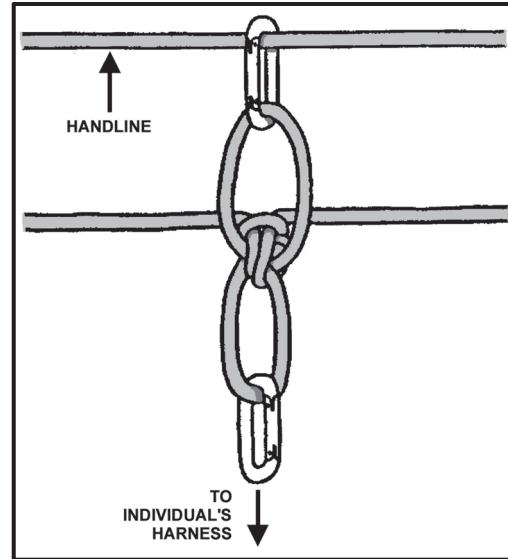
Figure 9-5. Belay rope for crossing using a handline.
