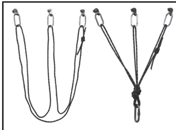
Figure 5-19. Pre-equalized anchor.
