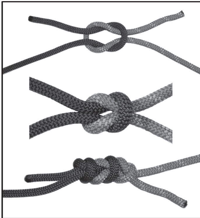
Figure 4-6. Square knot.
