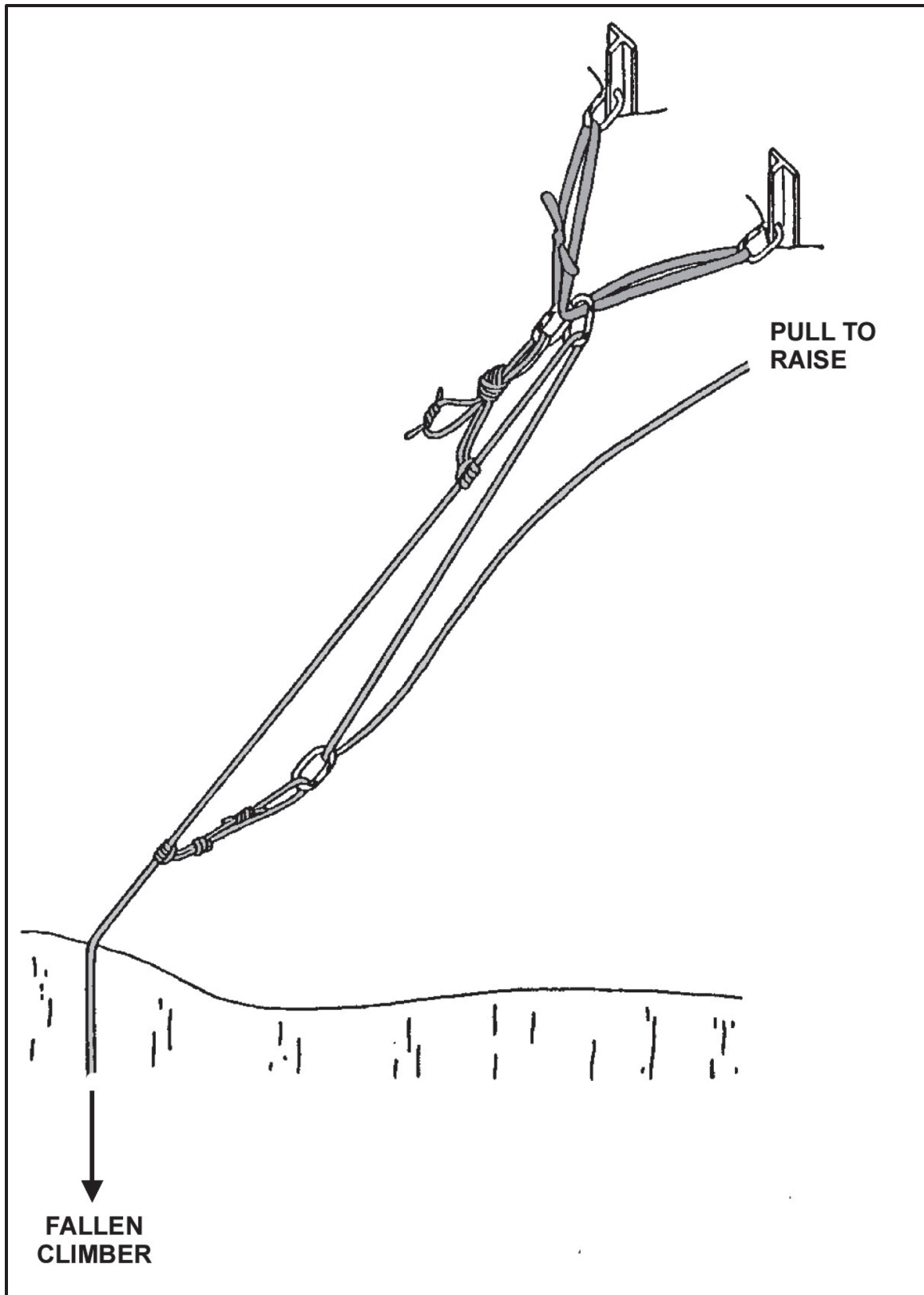
Figure 10-27. Z-pulley hauling system.
