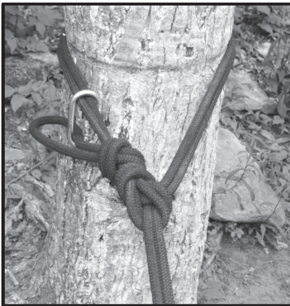
Figure 5-10. Rope tied to anchor with anchor knot.
