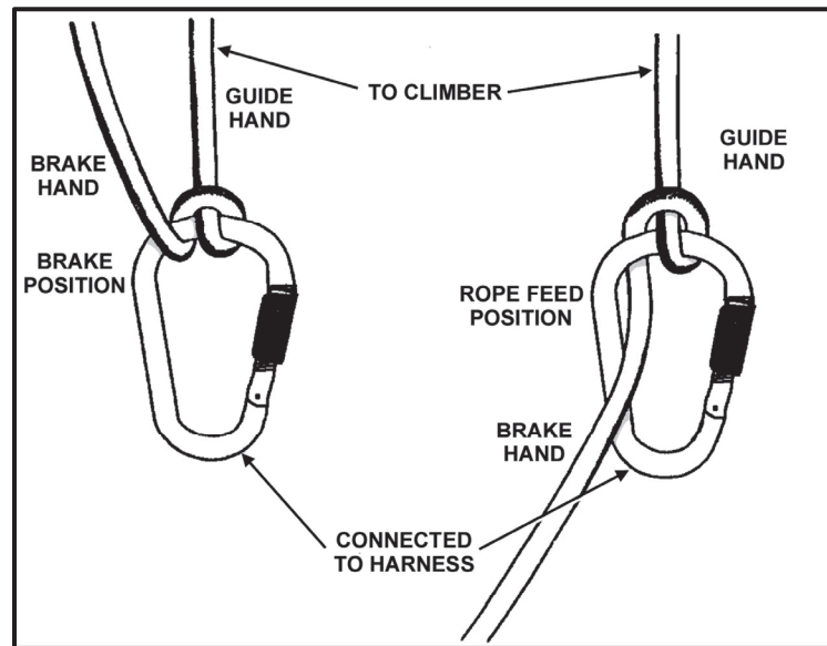
Figure 6-25. Munter hitch.
