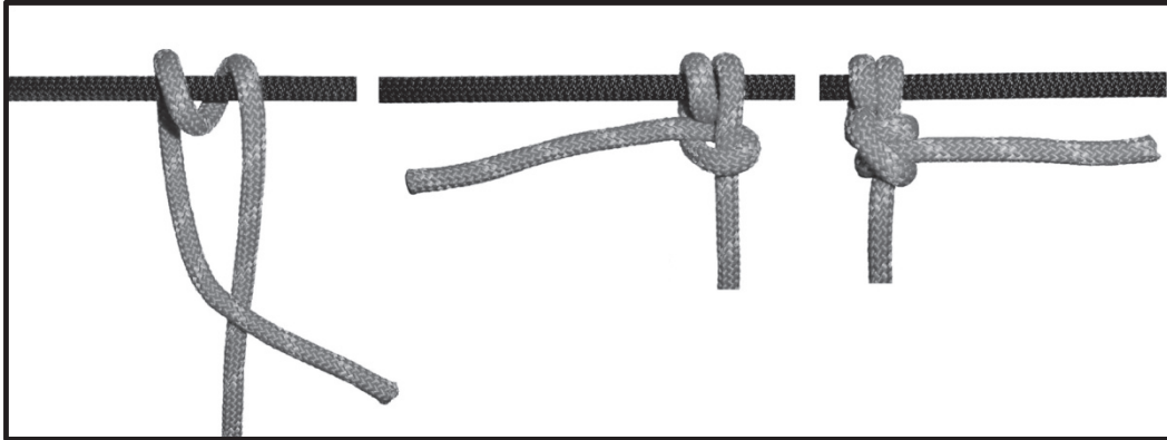
Figure 4-12. Round turn and two half hitches.
