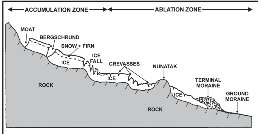
Figure 10-21. Glacier cross-section.
