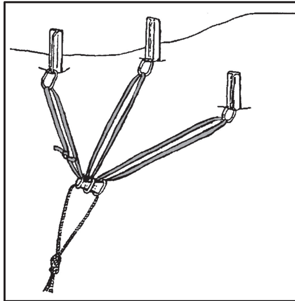
Figure 10-19. Equalized anchor using pickets.
