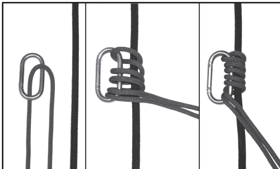
Figure 4-22. Bachman knot.
