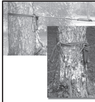
Figure 7-12. Round turn around anchor and two half hitches on a bight.
