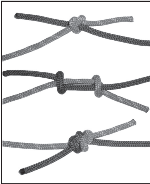
Figure 4-7. Fisherman's knot.
