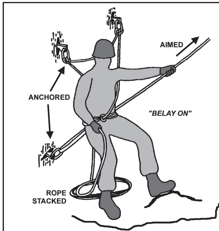
Figure 6-28. Belay setup.
