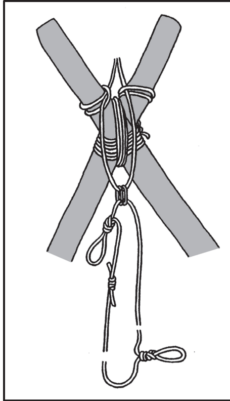
Figure 7-25. Attaching the anchor rope to the A-frame.
