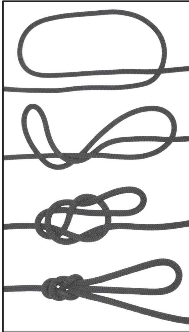
Figure 4-16. Directional figure eight.
