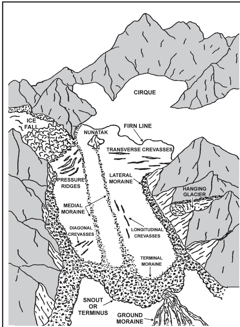
Figure 10-22. Glacier features.
