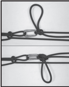
Figure 7-11. Transport knot.
