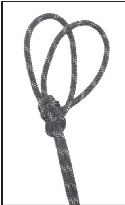
Figure 4-17. Bowline-on-a-bight.
