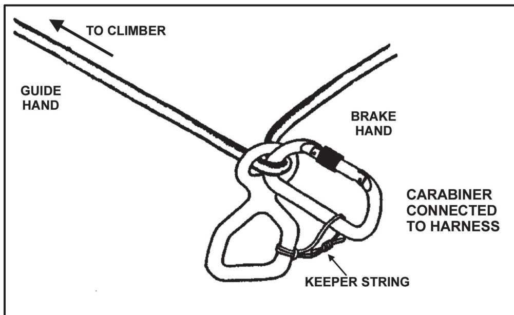
Figure 6-26. Figure-eight device.
