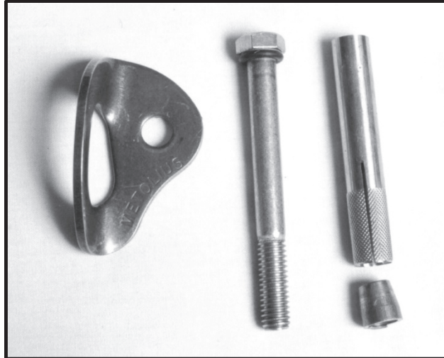
Figure 3-19. Bolts and hangers.
