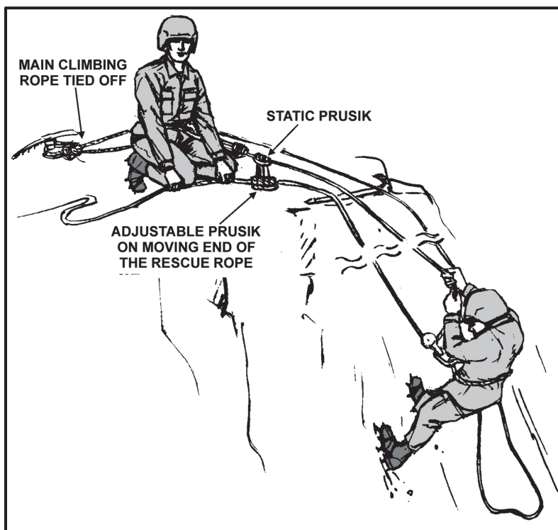
Figure 7-27. U-pulley system.
