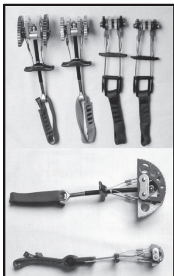
Figure 5-16. SLCD placements.
