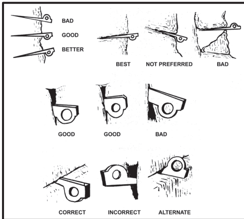
Figure 5-12. Examples of piton placements.
