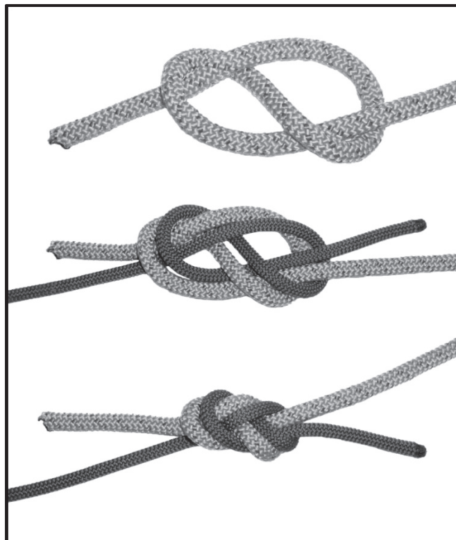
Figure 4-9. Figure-eight bend.
