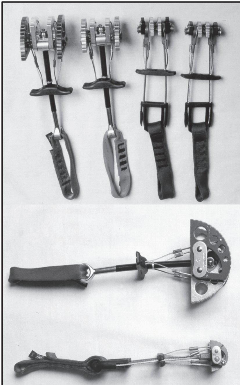
Figure 3-17. Spring-loaded camming devices.
