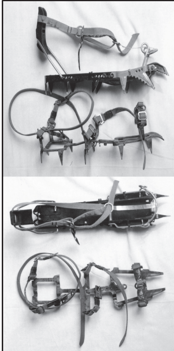
Figure 3-25. Crampons.
