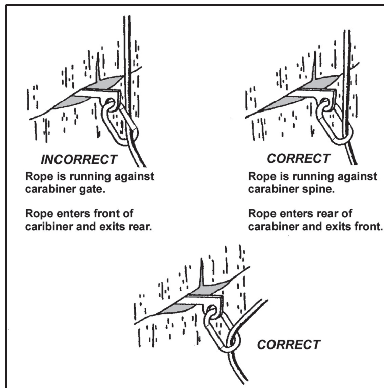
Figure 6-29. Clipping onto protection.
