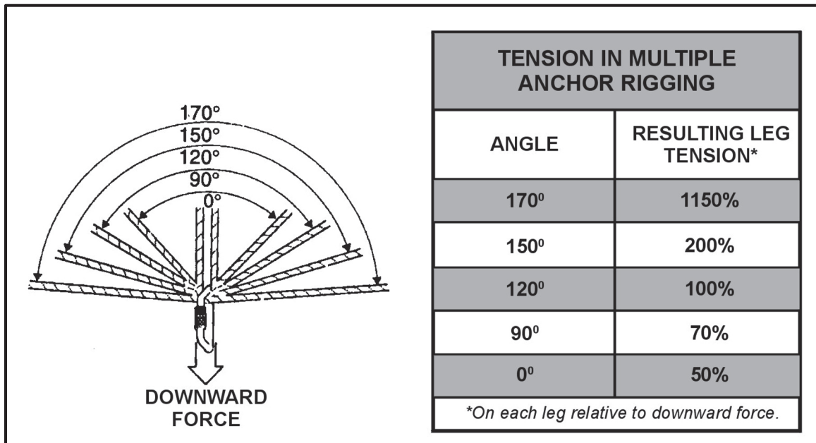
Figure 5-20. Effects of angles on an anchor.
