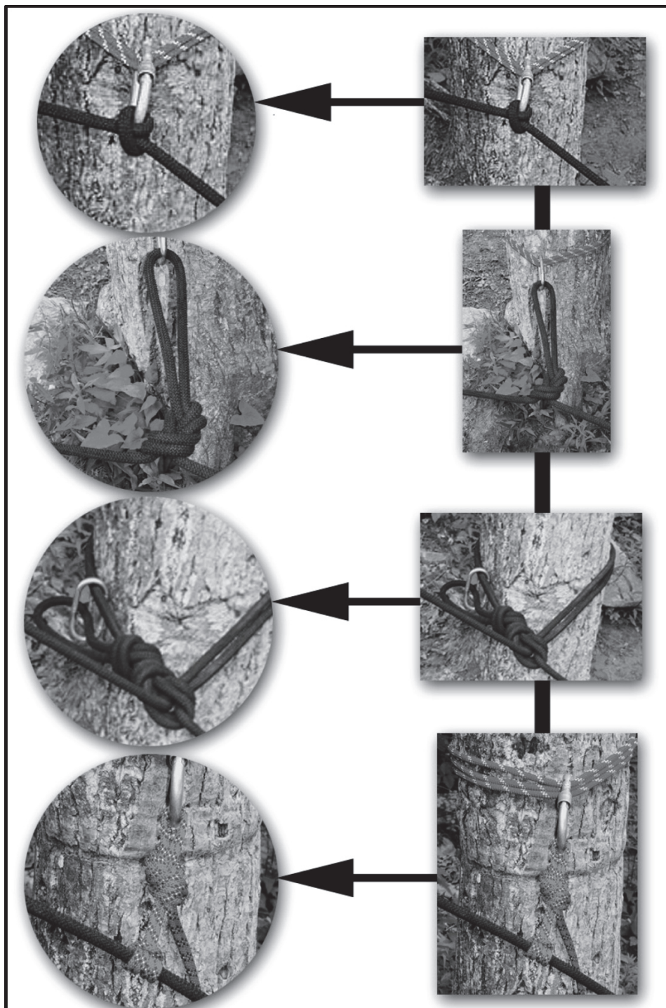
Figure 7-3. Fixed rope with intermediate anchors.
