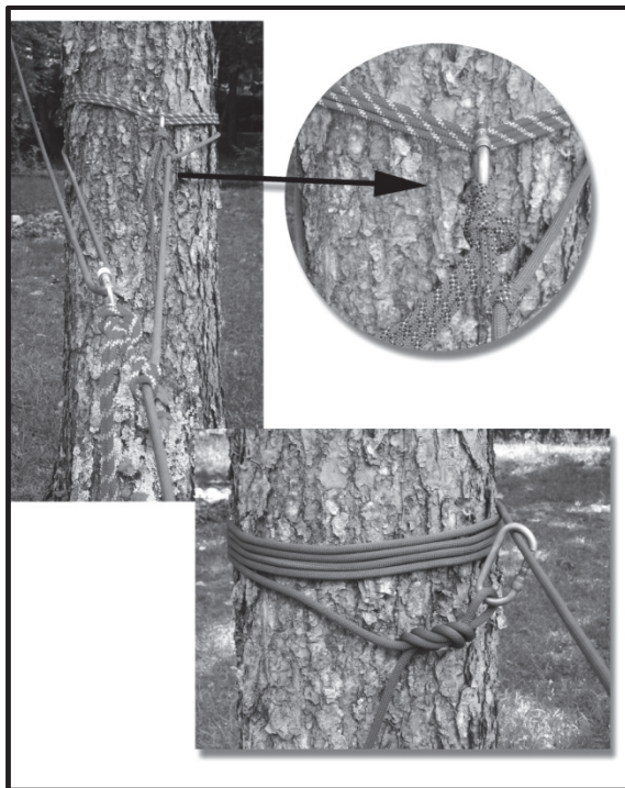
Figure 7-14. Z-pulley tightening system.
