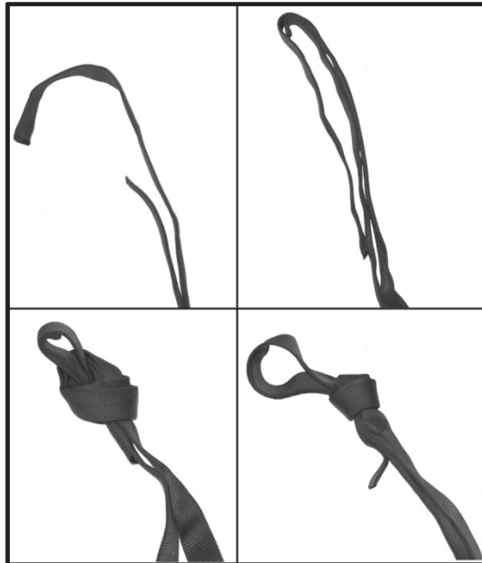
Figure 4-28. Frost knot.
