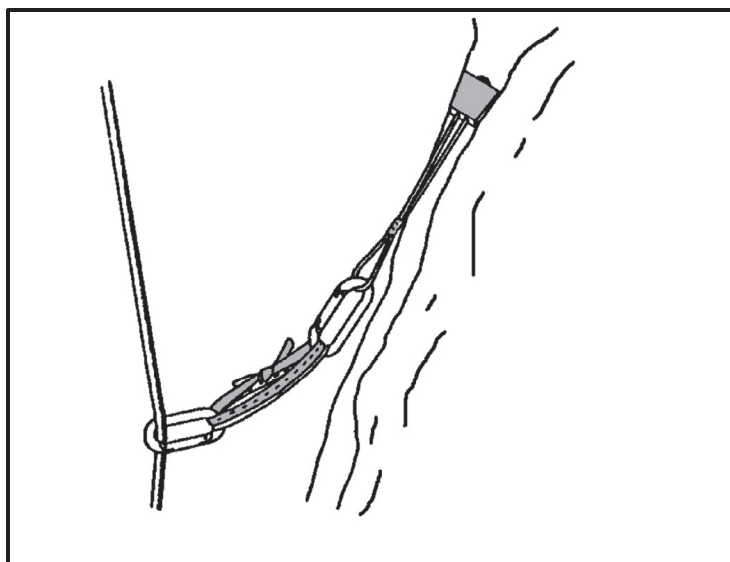
Figure 6-32. Use of sling on a wired stopper.
