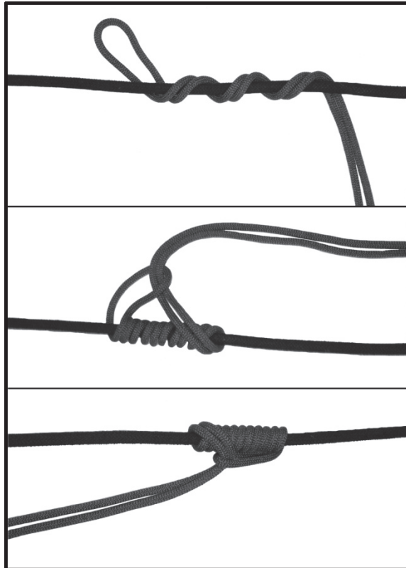
Figure 4-27. Kleimhiest knot.
