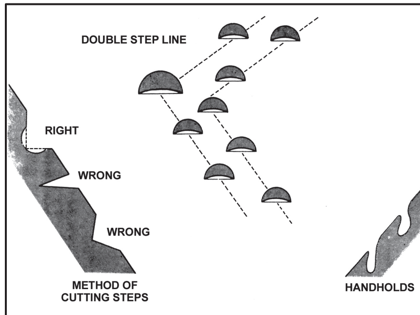
Figure 10-13. Step cutting and handhold cutting.
