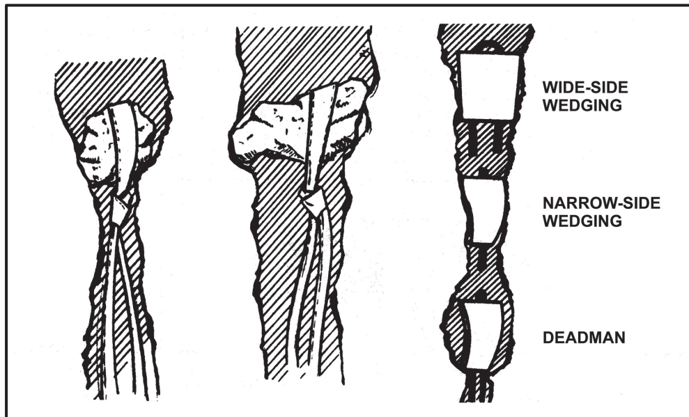
Figure 5-15. Chock placements.
