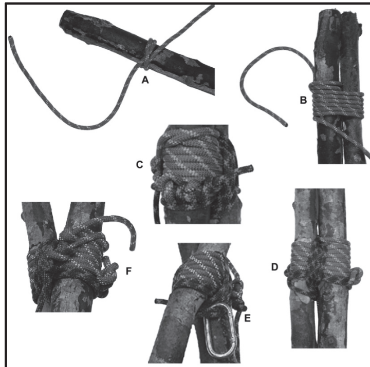
Figure 7-20. A-frame horizontal and vertical wraps.
