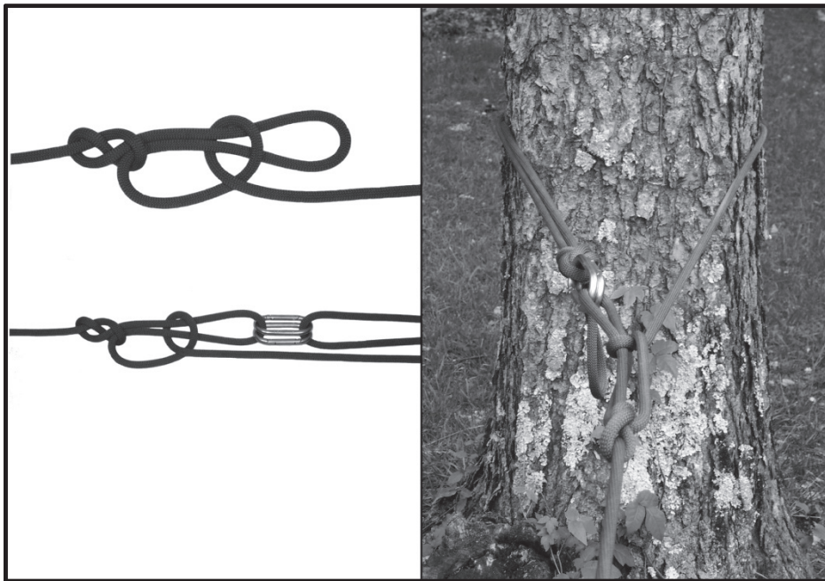
Figure 7-10. Transport tightening system.
