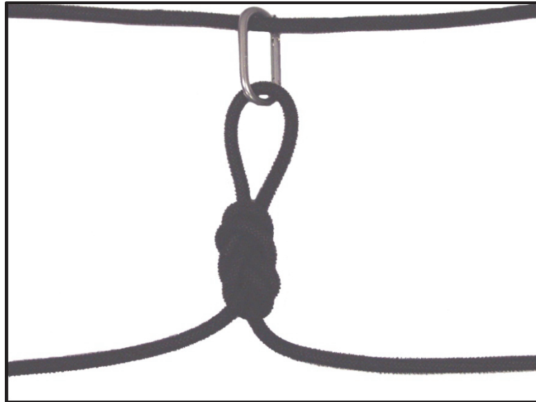
Figure 7-18. Hauling line.
