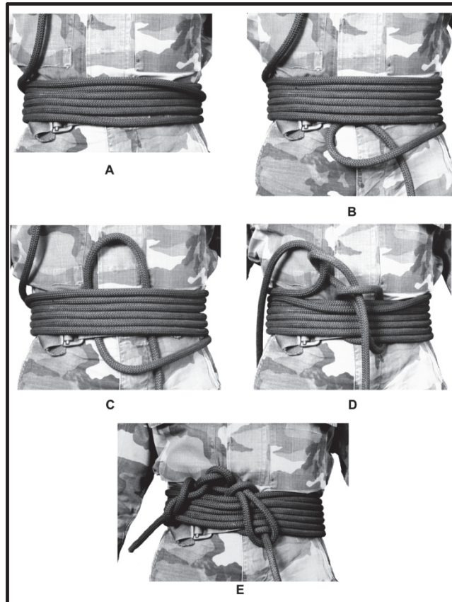
Figure 4-23. Bowline-on-a-coil.
