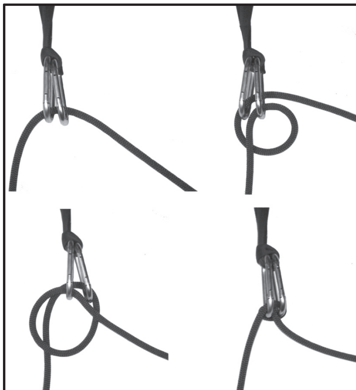
Figure 4-32. Garde knot.
